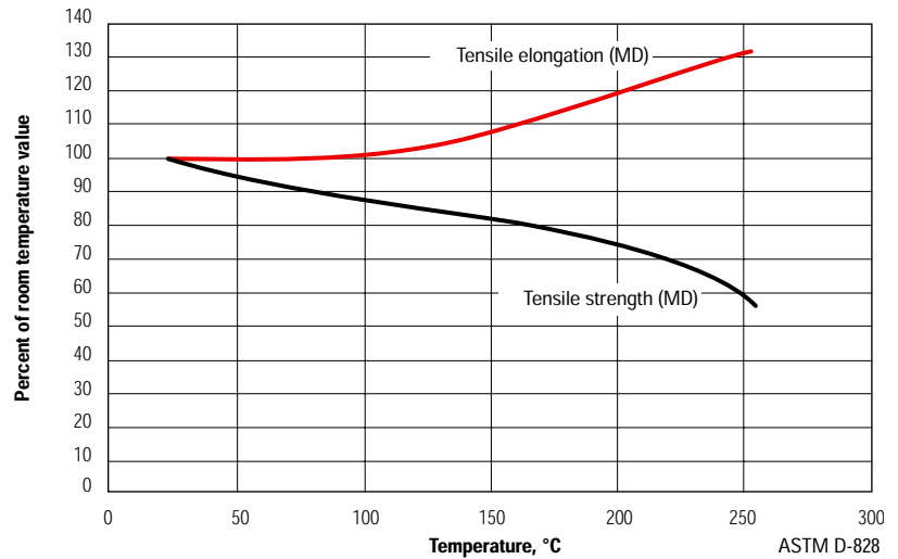
Figure 5 – EFFECT OF TEMPERATURE ON MECHANICAL PROPERTIES NOMEX® TYPE 410 – 0.25 MM (10 MIL)
